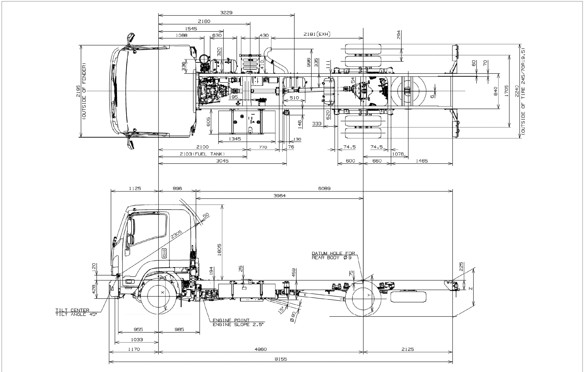
Fig. 9-1-2 Cab Chassis Drawing FSR34UL-NCUN
