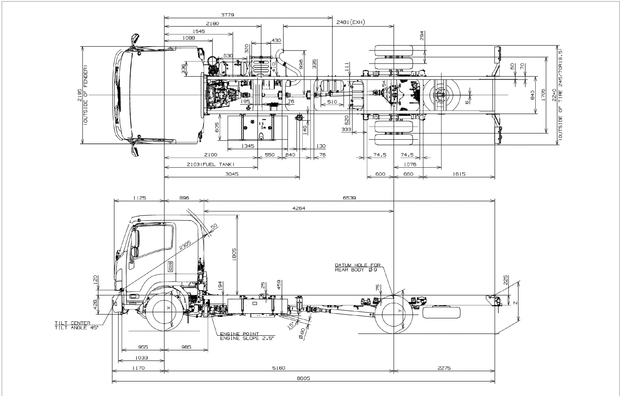
Fig. 9-1-3 Cab Chassis Drawing FSR34UL-PCUN
