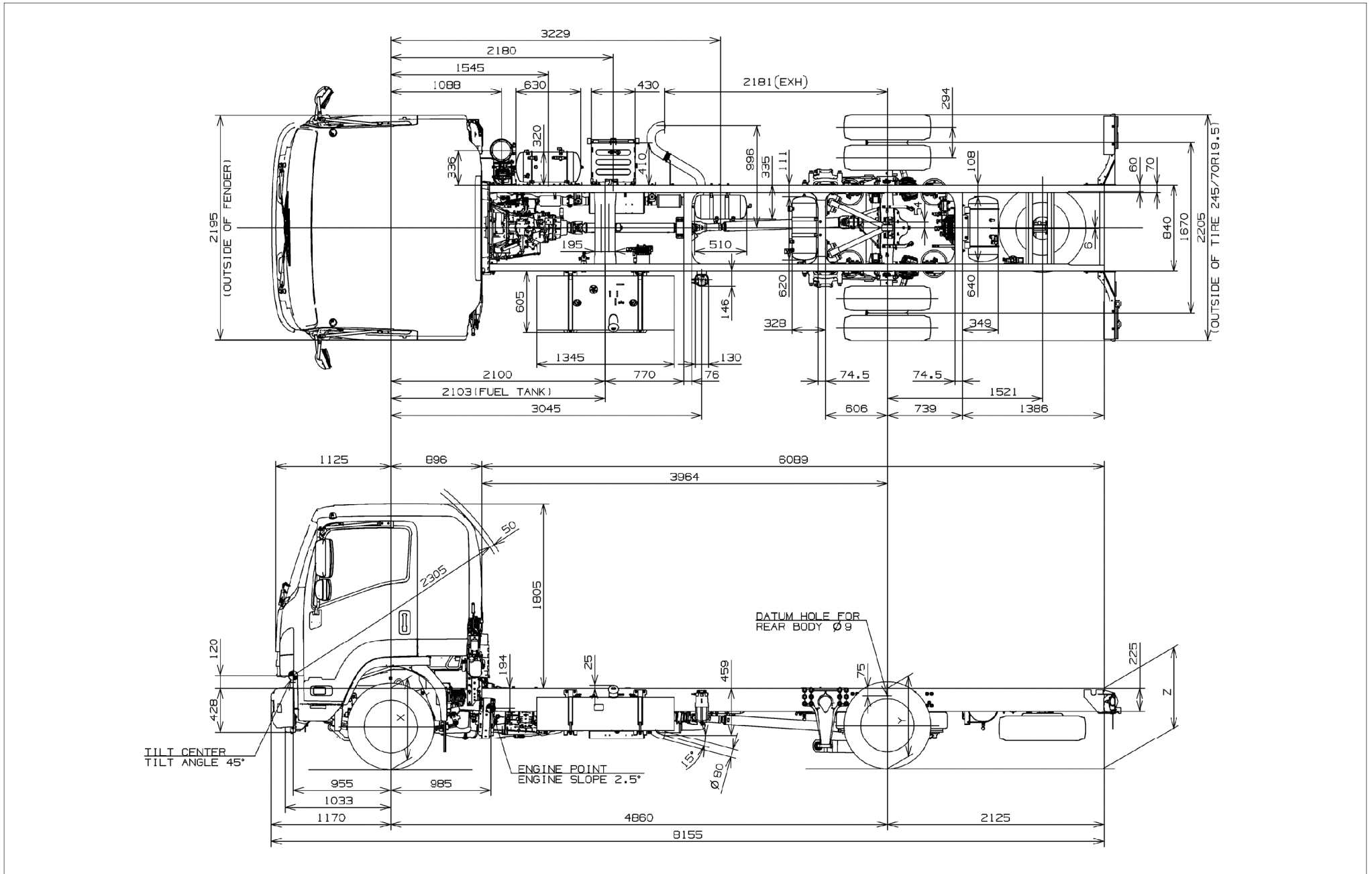
Fig. 9-1-4 Cab Chassis Drawing FSR34VL-NCUN
