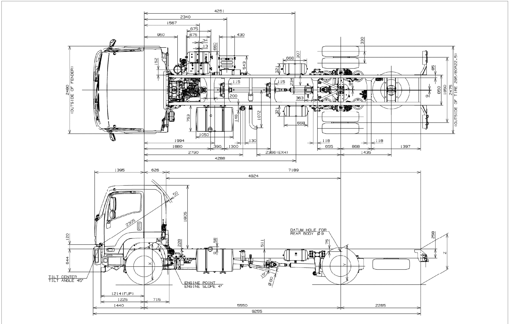
Fig. 9-1-10 Cab Chassis Drawing FVR34VL-QDUC
