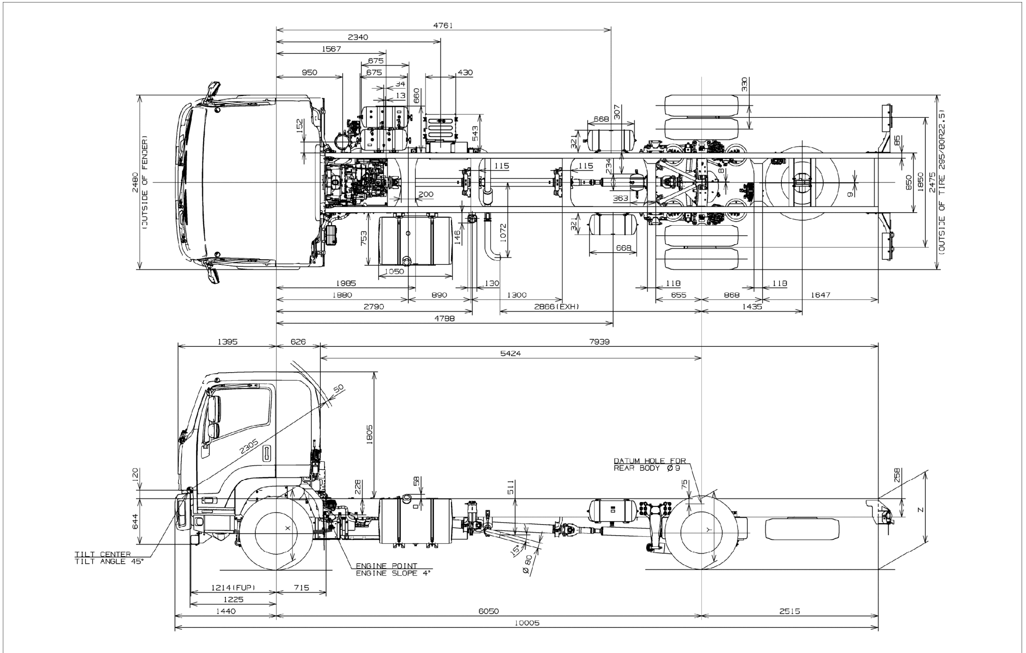
Fig. 9-1-11 Cab Chassis Drawing FVR34VL-SDUC
